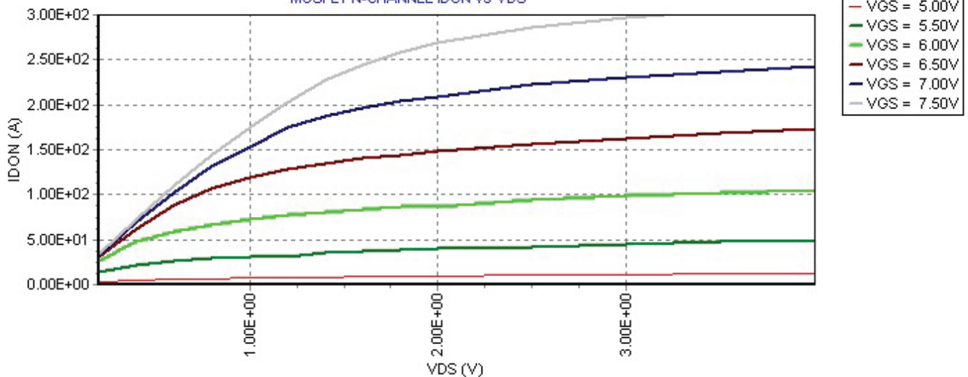
MOSFET N-CHANNEL IDON vs VDS
